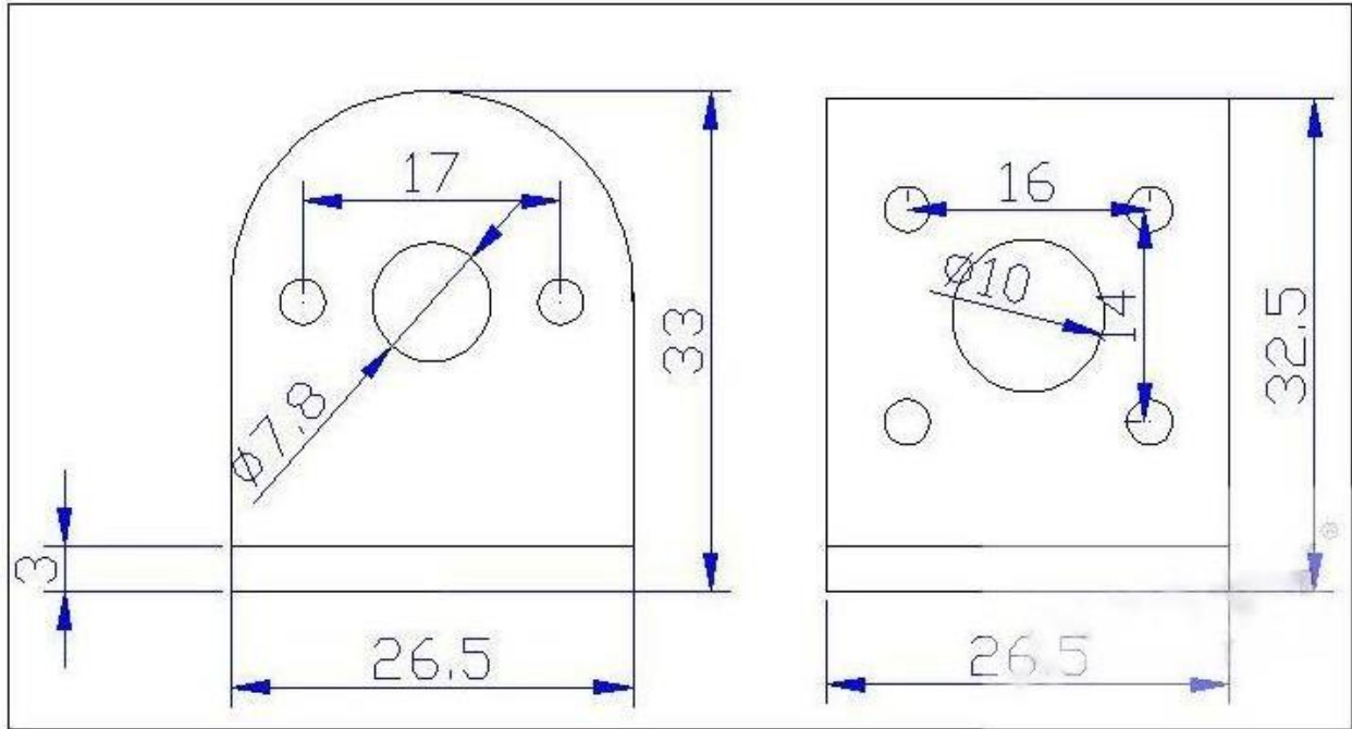
Fig. 1 Fixation Size
