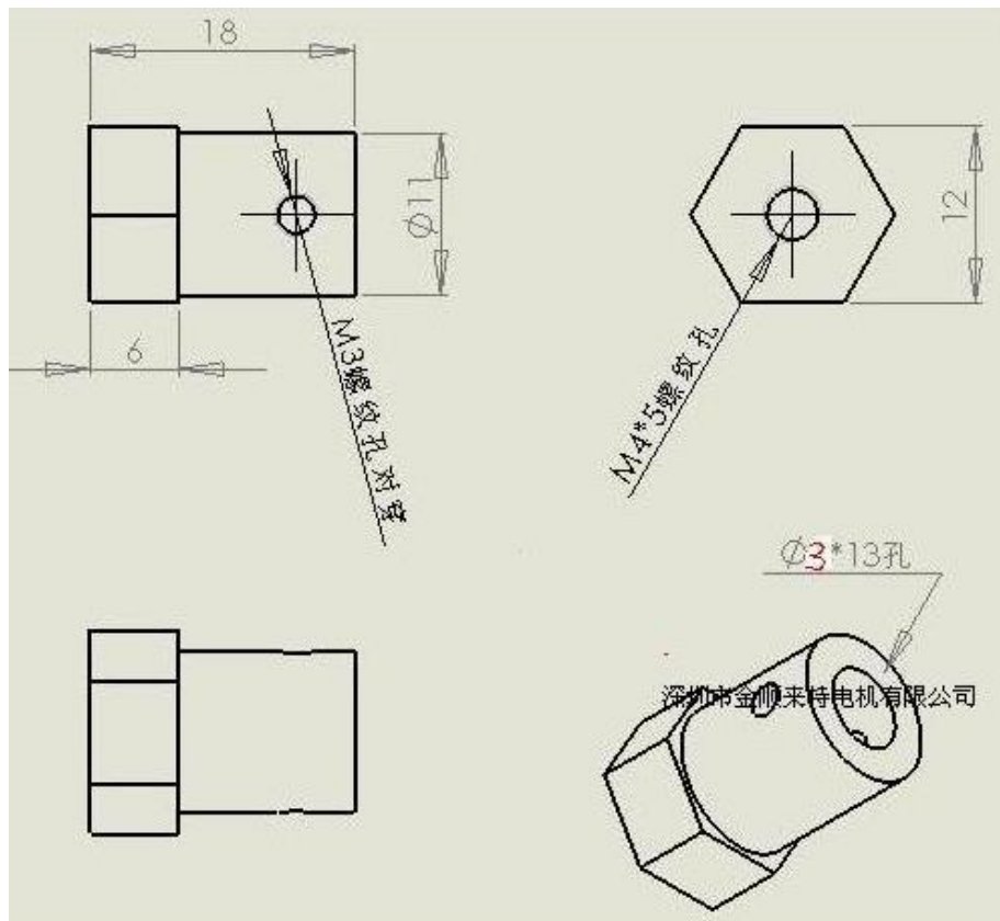
Fig. 2 Coupling Size
