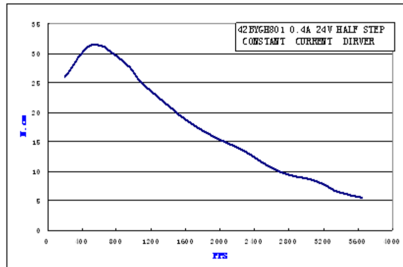
Pulse-Torque Characteristic
